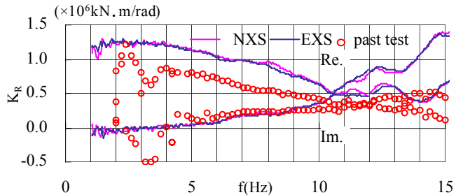
Fig. 11 Comparison of rocking spring by TEST20 and TEST21
