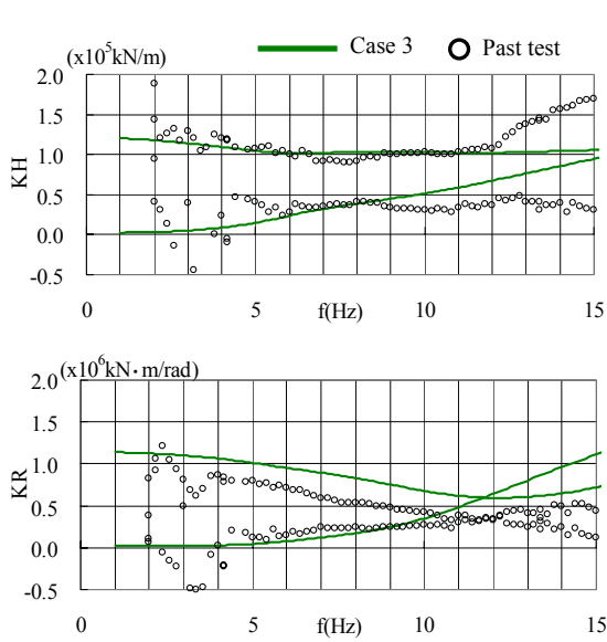
Fig.14 Comparison of sway and rocking springs between prediction analysis and TEST20
