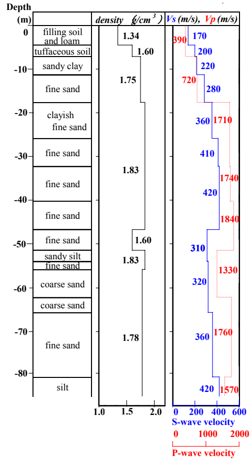
Fig. 2 Soil profile
