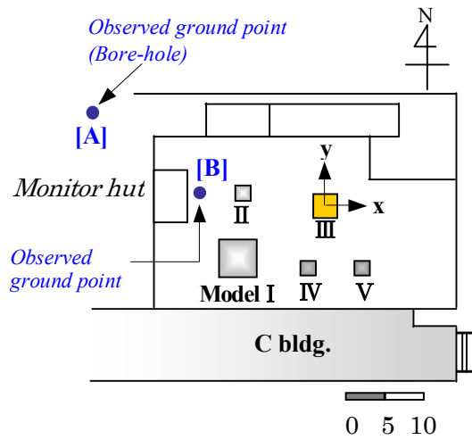
Fig. 1 Illustration of test field
