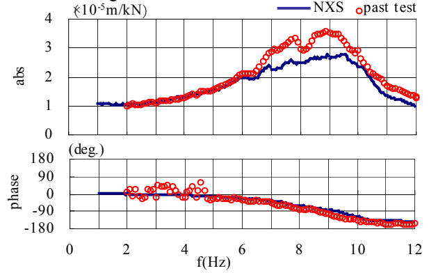
Fig. 9 Comparison of resonance curves ( U_T/P ) by past and TEST2001 (no-added weight)
