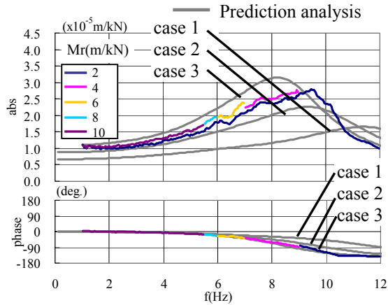
Fig. 7 Comparison of displacement resonance curves ( U_T/P ) between prediction analyses and TEST21(no-added weight)
