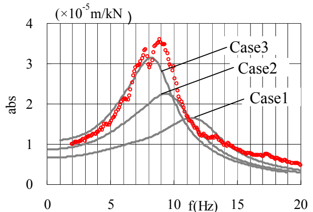
Fig. 6 Displacement resonance curves ( U_T/P ) by prediction analysis
