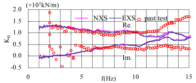
Fig. 10 Comparison of sway spring by TEST20 and TEST21
