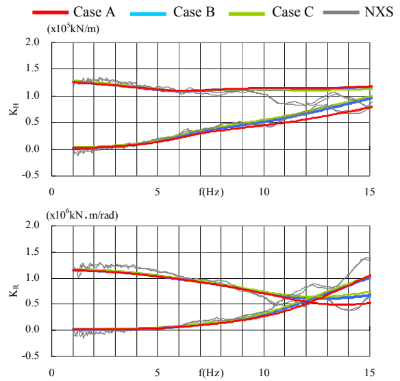
Fig.15 Comparison of sway and rocking springs between numerical analysis and TEST21
