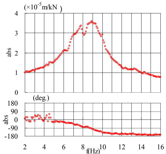
Fig. 4 Displacement resonance curves of Model III of TEST20
