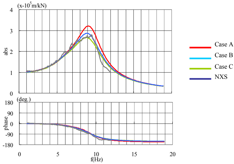
Fig.13 Comparison of displacement resonance curves ( U_T/P ) between numerical analysis and TEST21
