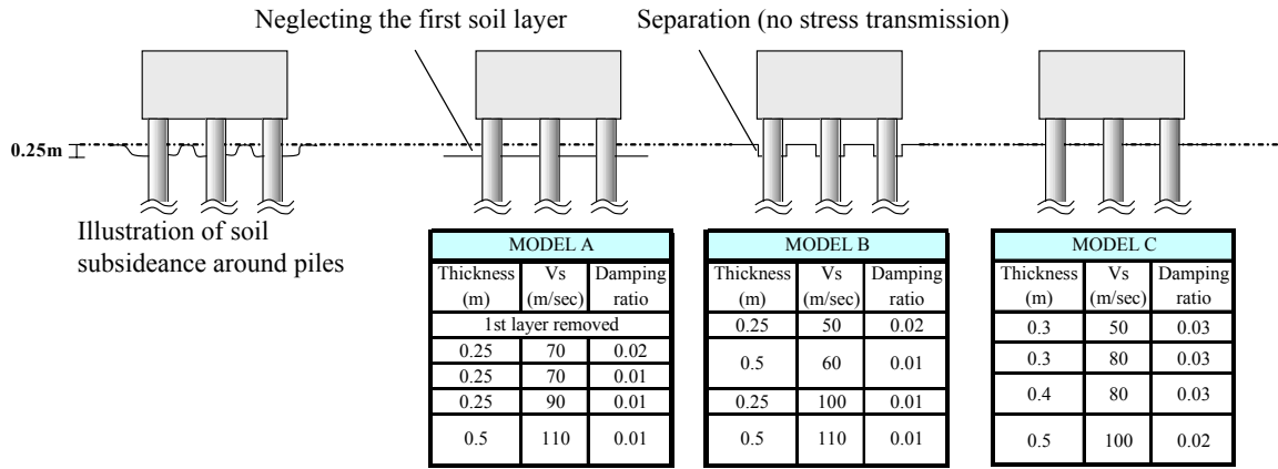
Fig.12 Numerical analysis cases
