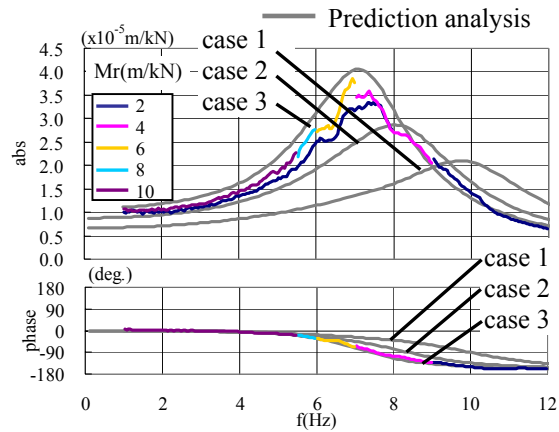
Fig. 8 Comparison of displacement resonance curves ( U_T/P ) between prediction analyses and TEST20(added weight)
