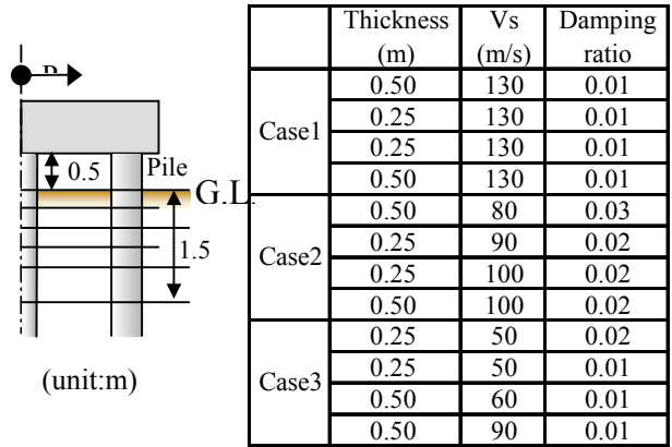
Fig. 5 Prediction analysis cases
